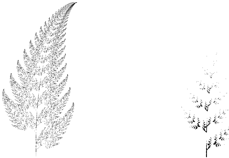
Figure I.12 – A gauche : p_1 = 0.01, p_2 = 0.07, p_3 = 0.07, p_4 = 0.85 , à droite : p_i = 0.25, i = 1, \dots, 4
