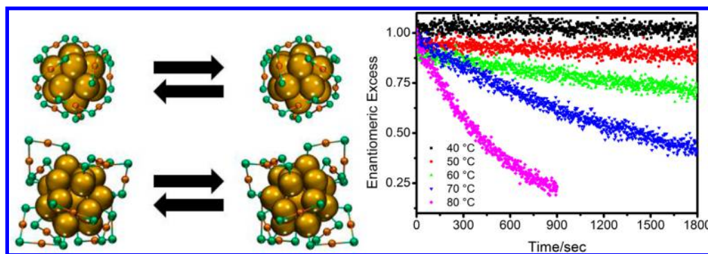
Figure 7. Left: Inversion reaction of \text{Au}_{38}(\text{SR})_{24} (top) and \text{Au}_{40}(\text{SR})_{24} (bottom). Right: Evolution of the enantiomeric excess of \text{Au}_{38}(2\text{-PET})_{24} at different temperatures. Acceleration of the racemization is observed for higher temperatures. Data were originally published in ref 52.
