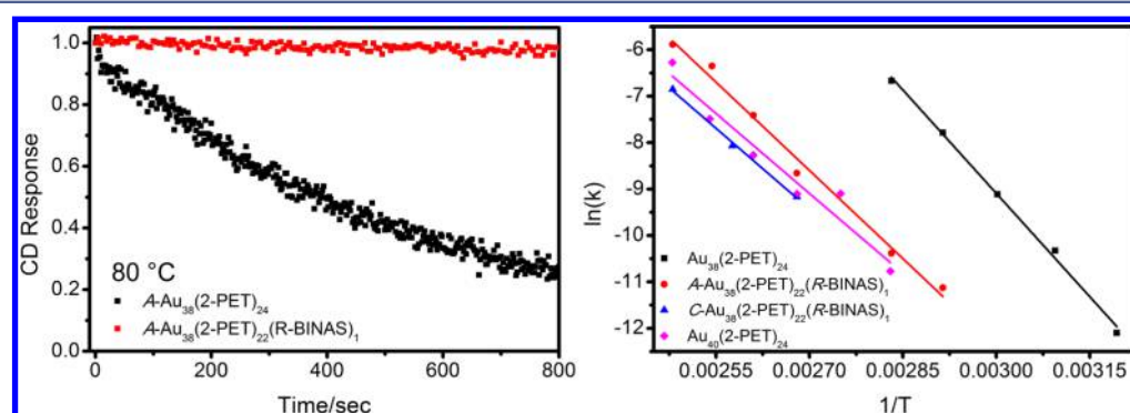
Figure 9. Left: Normalized optical activity of \text{Au}_{38}(\text{2-PET})_{24} and \text{A-Au}_{38}(\text{2-PET})_{22}(\text{R-BINAS})_1 at 80 °C. While the unsubstituted cluster shows fast decrease of optical activity (black), BINAS-substitution leads to almost constant values (red). Right: Arrhenius plots for \text{Au}_{38}(\text{2-PET})_{24} (black), \text{A-Au}_{38}(\text{2-PET})_{22}(\text{R-BINAS})_1 (red), \text{C-Au}_{38}(\text{2-PET})_{22}(\text{R-BINAS})_1 (blue), and \text{Au}_{40}(\text{2-PET})_{24} (magenta). The data were originally published in refs 52, 63, and 53.
