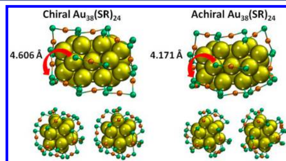
Figure 4. Top: Chiral (left) and achiral (right) structures of \text{Au}_{38}(\text{SR})_{24} in comparison (coordinates from ref 46). Marked with arrows are one sulfur atom of one monomeric unit and the nearest sulfur atom from a neighboring dimeric unit. The average distances over the cluster are assigned. Bottom: Views along the principal axis of the isomers in both directions. The chiral structure shows the same handedness; the achiral structure shows opposite handedness.
