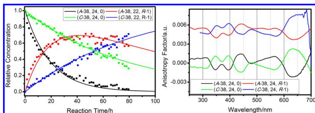
Figure 8. Left: Concentration profiles of the ligand exchange reaction of A- and C- \text{Au}_{38}(\text{2-PET})_{24} (black and green) with R-BINAS. The left-handed cluster reacts much faster than the right-handed enantiomer. Right: Anisotropy factors of \text{Au}_{38}(\text{2-PET})_{24} and \text{Au}_{38}(\text{2-PET})_{22}(\text{R-BINAS})_1 . The spectra of the diastereomers (red and blue) resemble those of the unsubstituted enantiomers (black, green). Data were originally published in refs 63 and 76.
