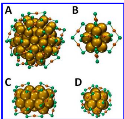
Figure 3. Crystal structure of the \text{Au}_{102}(\text{p-MBA})_{44} cluster (A), \text{Au}_{25}(\text{2-PET})_{18} (B), and \text{Au}_{38}(\text{2-PET})_{24} in side-view (C) and along its principal axis (D). For the latter, the left-handed A -enantiomer is shown. The organic groups are removed. Atomic positions are from refs 13, 14, and 16. Yellow, \text{Au}_{\text{Core}} ; orange, \text{Au}_{\text{Atom}} ; green, sulfur.
