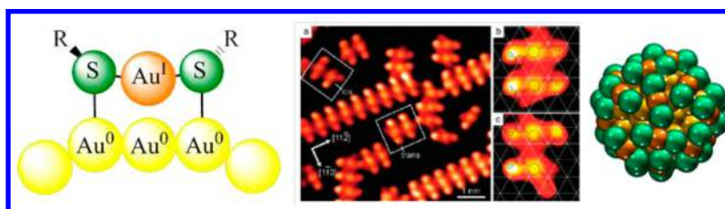
Figure 2. Protecting units in thiolate-protected gold clusters and on extended surfaces. Left: schematic of a (short) SR-Au-SR unit. Middle: STM image of methylthiolate on a Au(111) surface. Reprinted with permission from ref 18. Copyright 2009 American Chemical Society. Right: crystal structure of the \text{Au}_{102}(\text{p-MBA})_{44} cluster (ref 13; the organic rest is not shown). The Au atoms in the schematics are colored according to their oxidation state.
