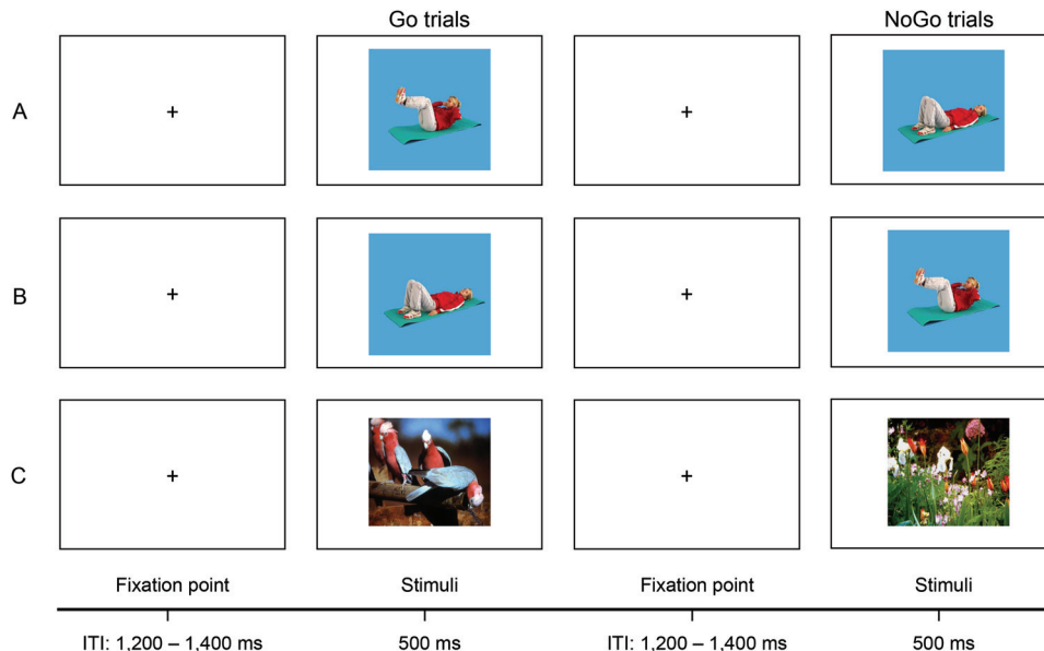
Figure 1 Go/No-Go Tasks
