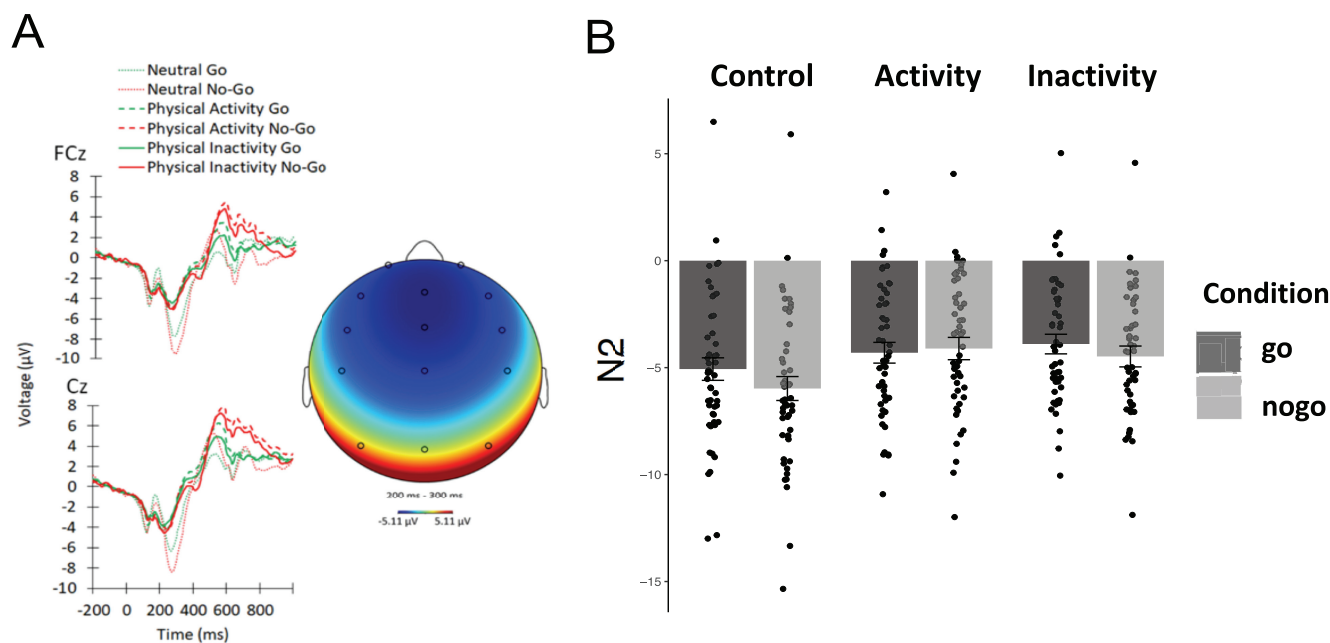
Figure 3 N2 Outcomes
