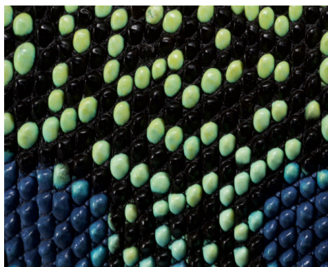
Detail of the scales that continue flipping colour during the lifetime of the animal.
