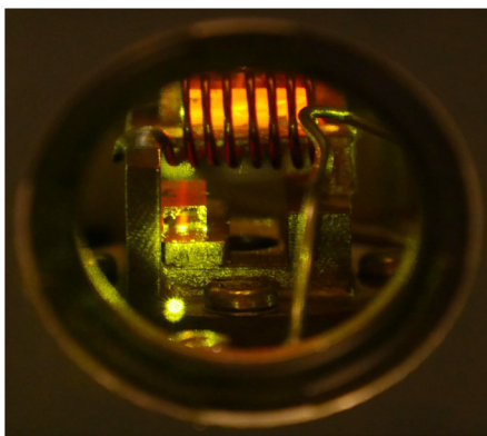
The quantum repeater: two crystals in operation.
